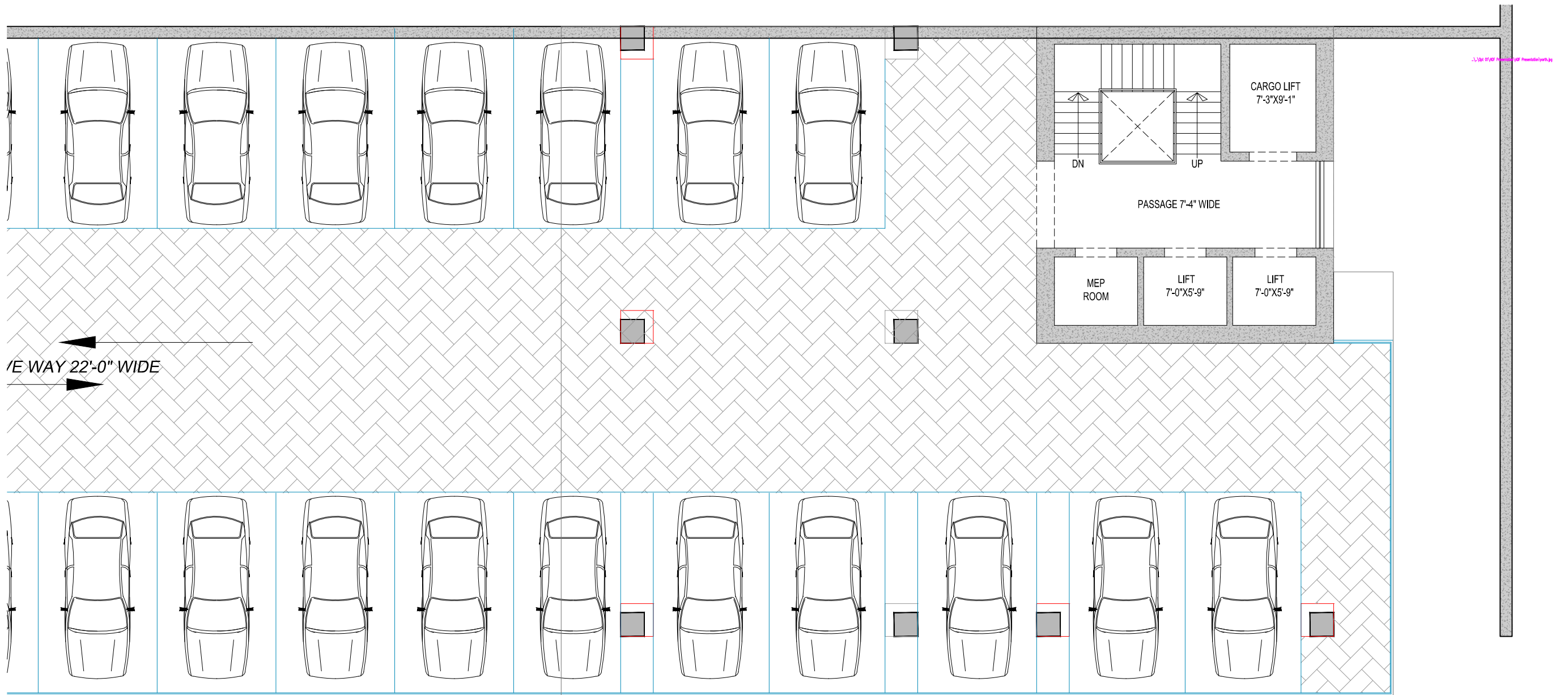
STAGE 01 3RD FLOOR PLAN
