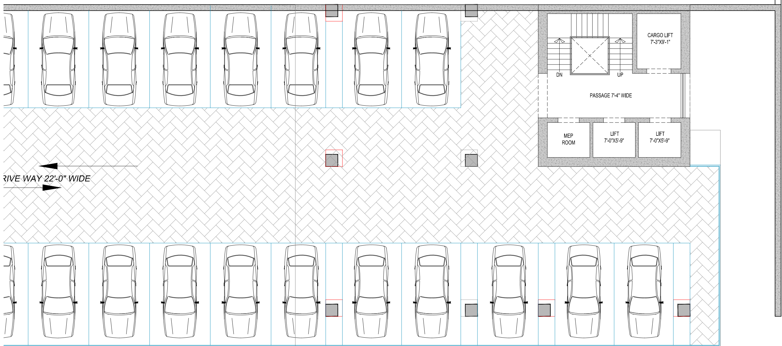
STAGE 01 1ST FLOOR PLAN
