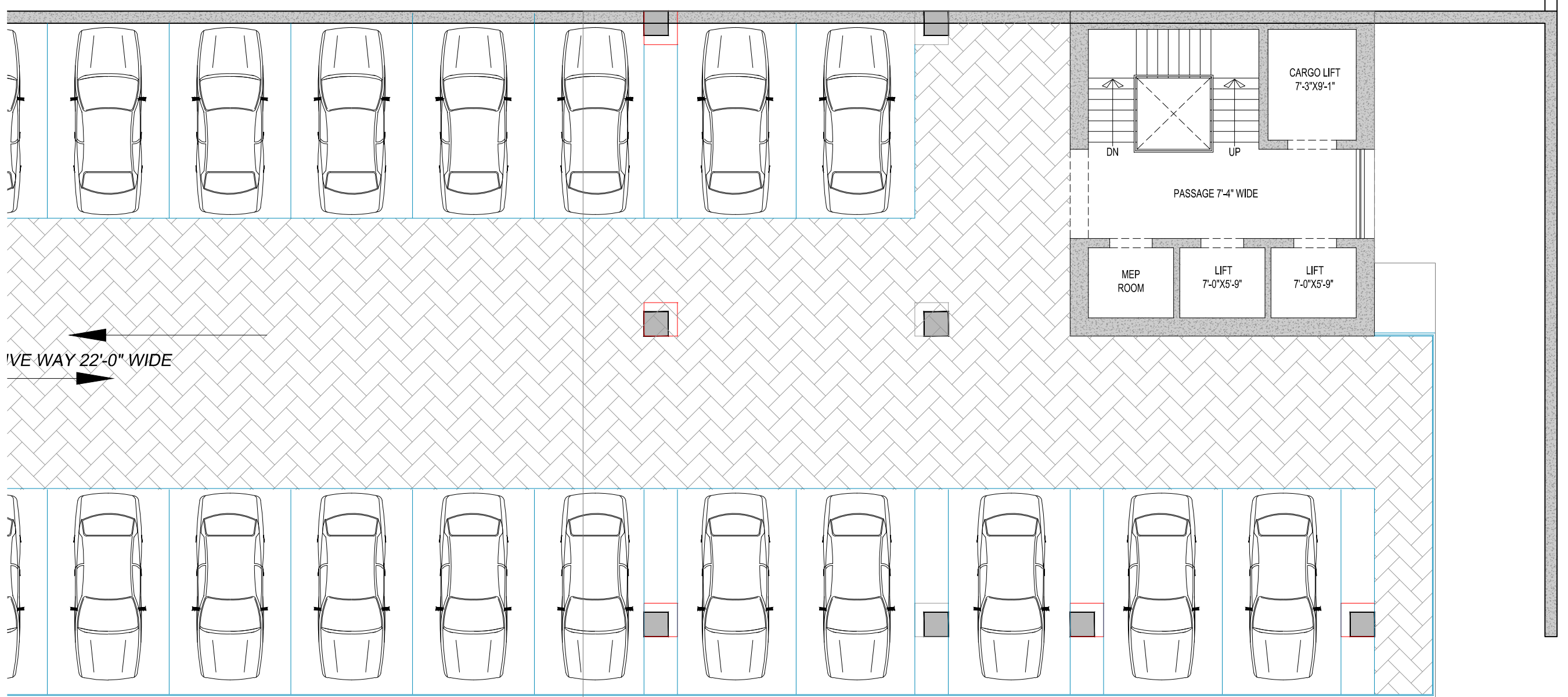
STAGE 01 2ND FLOOR PLAN
