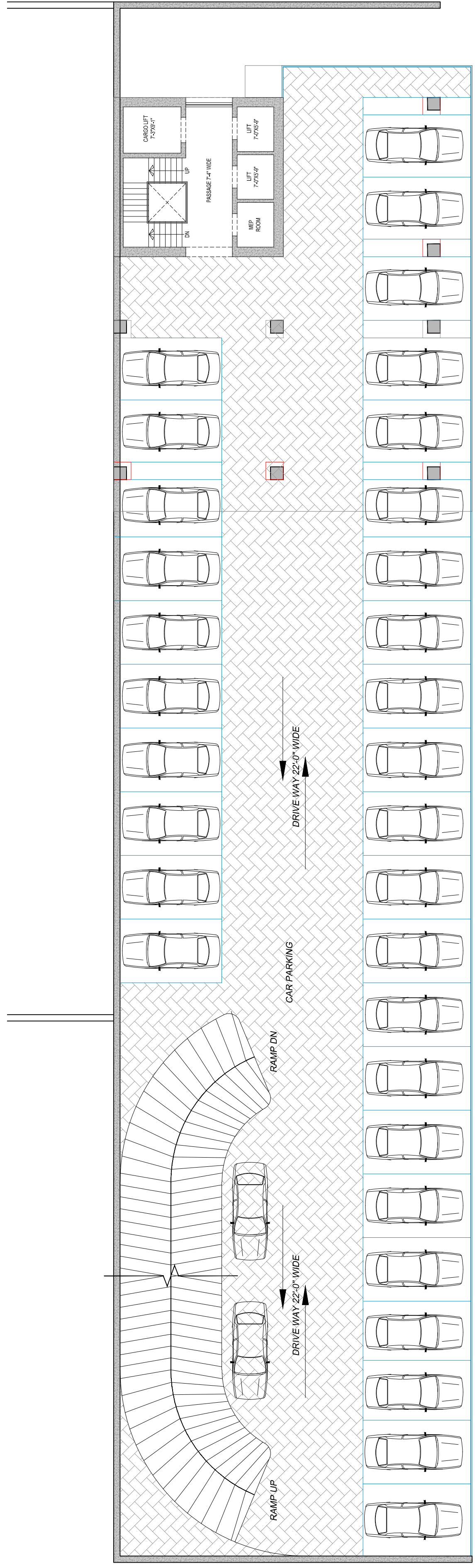
STAGE 01 2ND FLOOR PLAN
