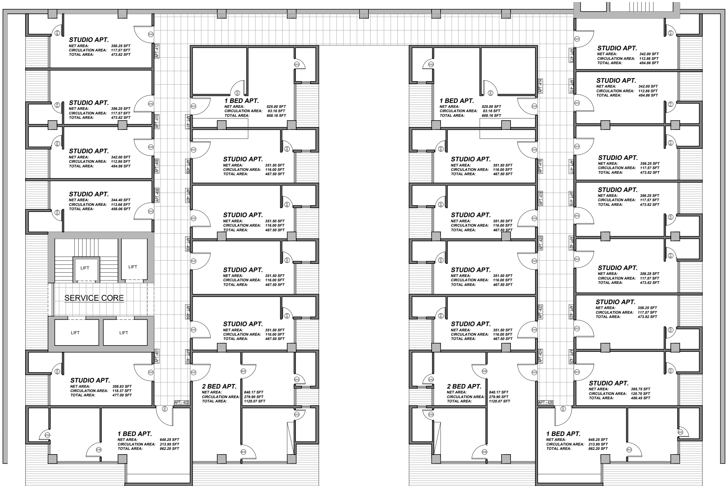
STAGE 02 4TH FLOOR AREA PLAN
