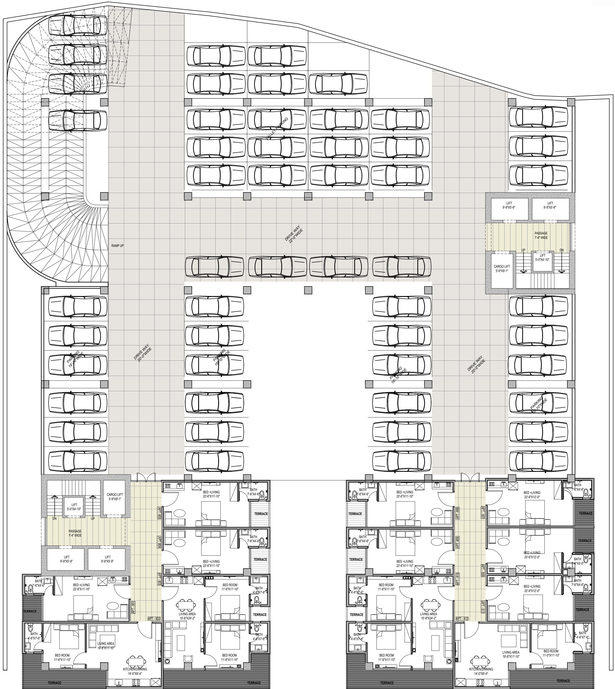
STAGE 03 8TH FLOOR PLAN 52 NO OF CARS
