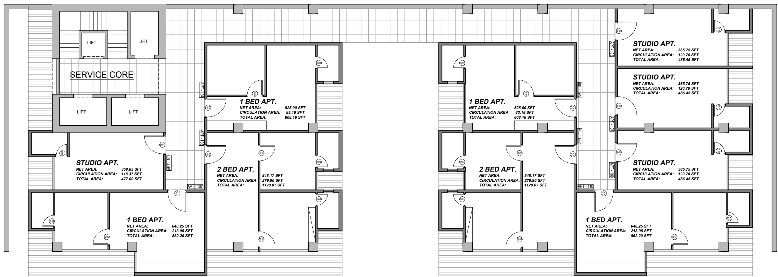
STAGE 01 1ST FLOOR AREA PLAN
