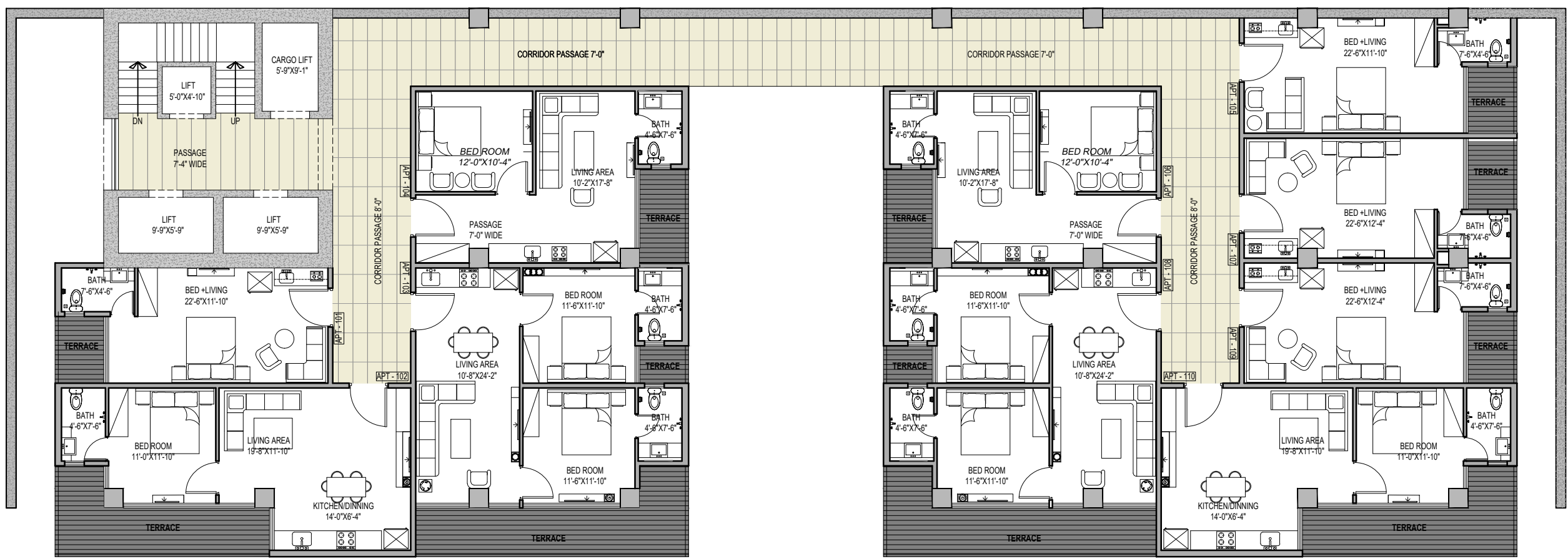
STAGE 01 FIRST FLOOR PLAN
