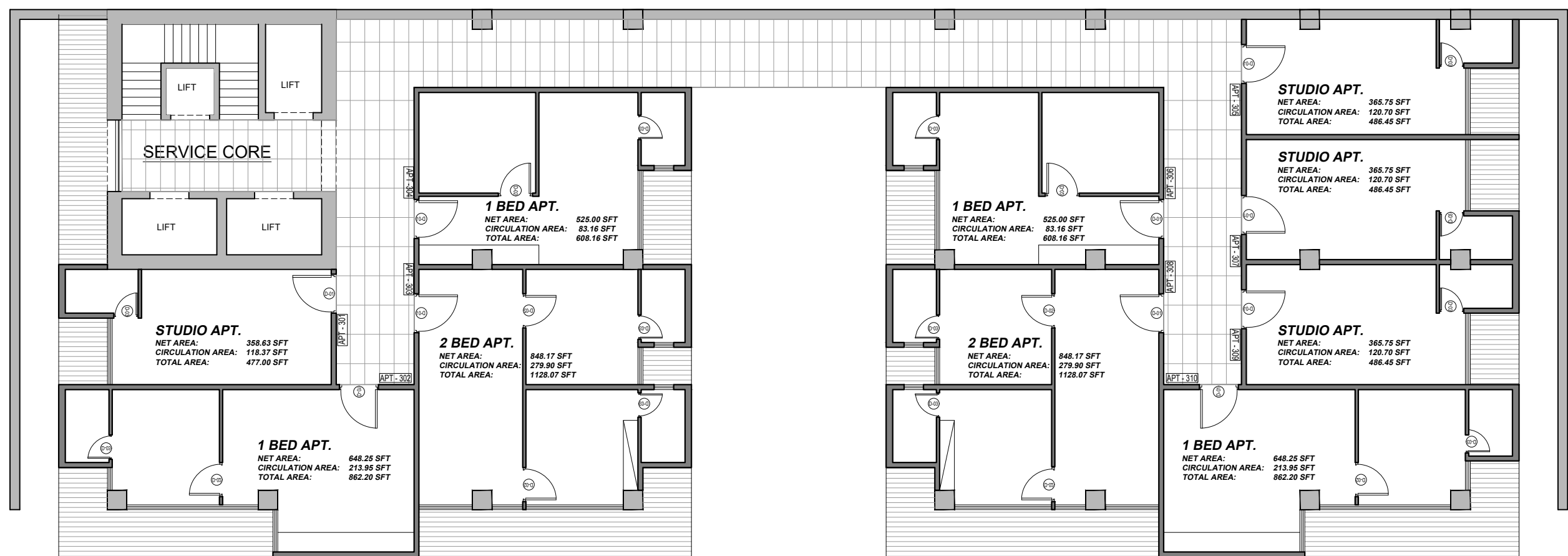
STAGE 01 3RD FLOOR AREA PLAN
