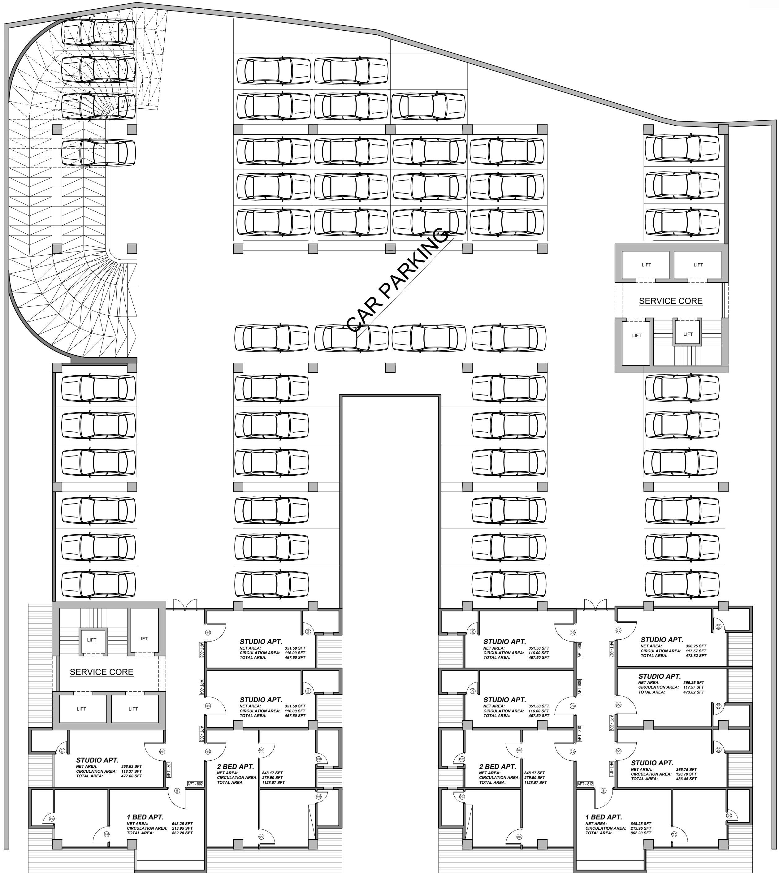
STAGE 03 8TH FLOOR AREA PLAN
