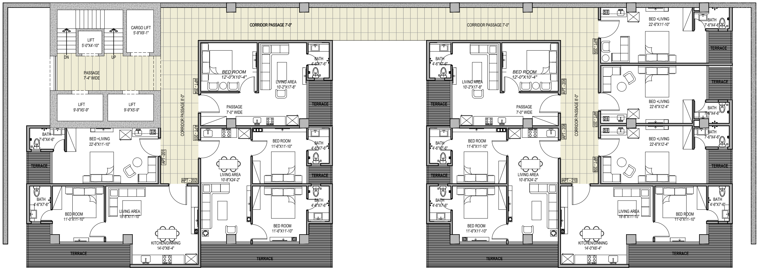
STAGE 01 2ND FLOOR PLAN
