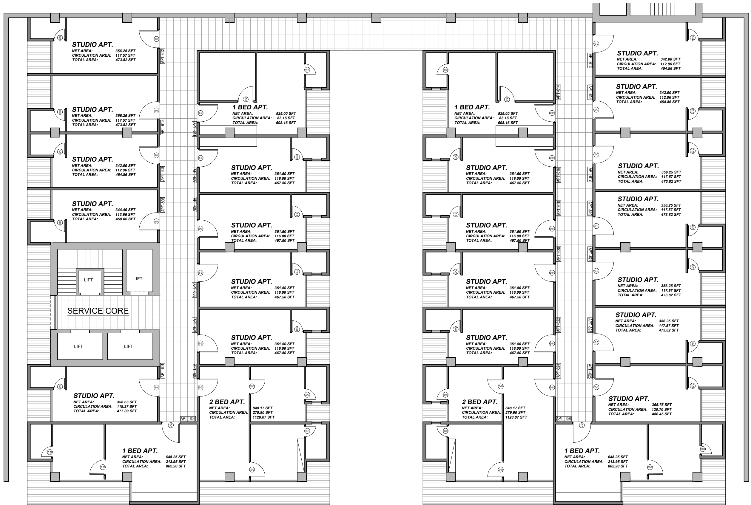
STAGE 02 6TH FLOOR AREA PLAN
