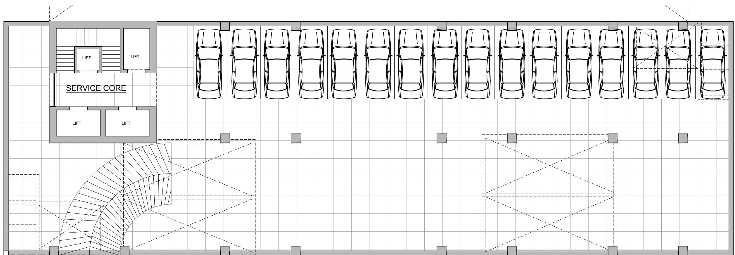
STAGE 01 LOWER GROUND FLOOR AREA PLAN
