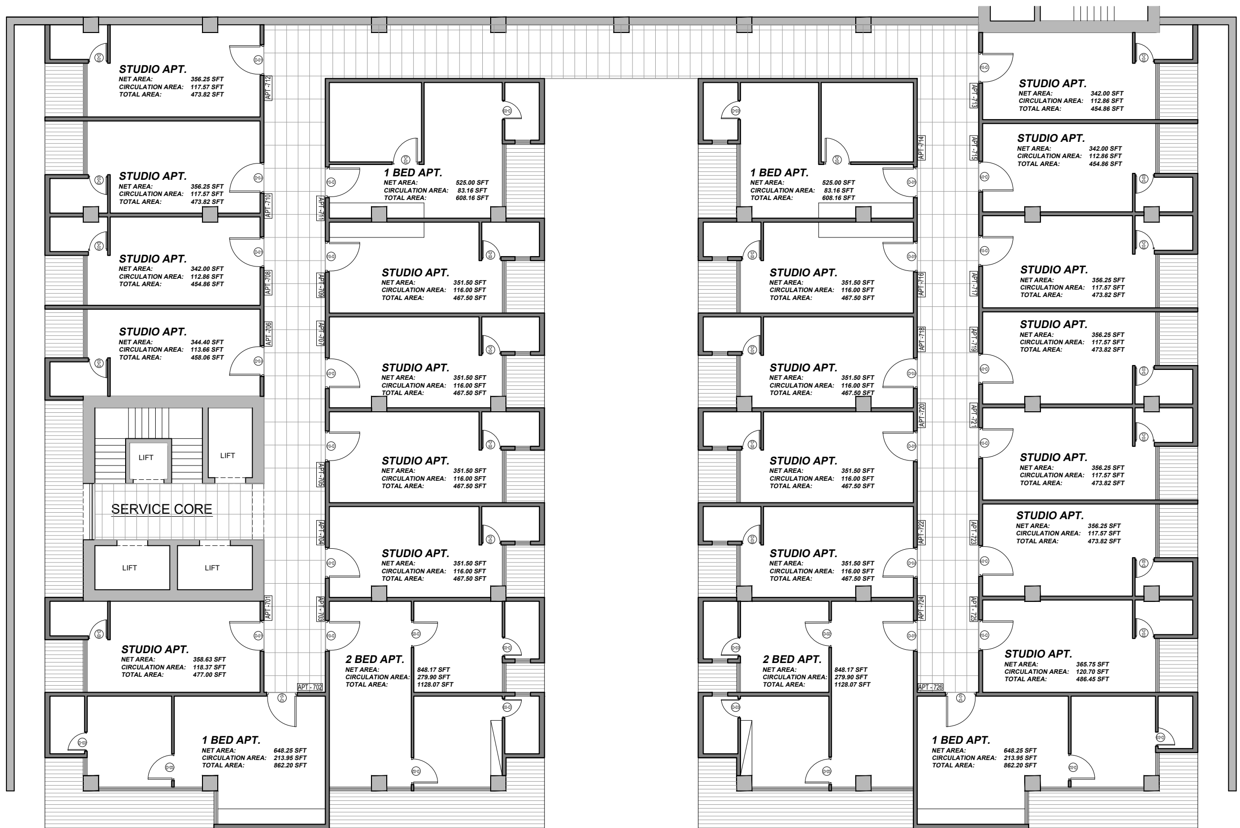
STAGE 02 7TH FLOOR AREA PLAN
