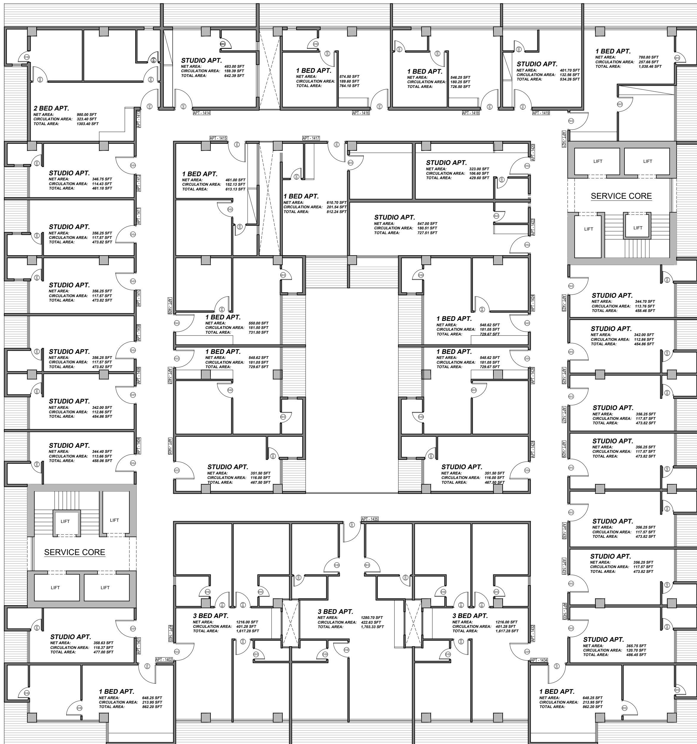
STAGE 03 14TH FLOOR AREA PLAN
