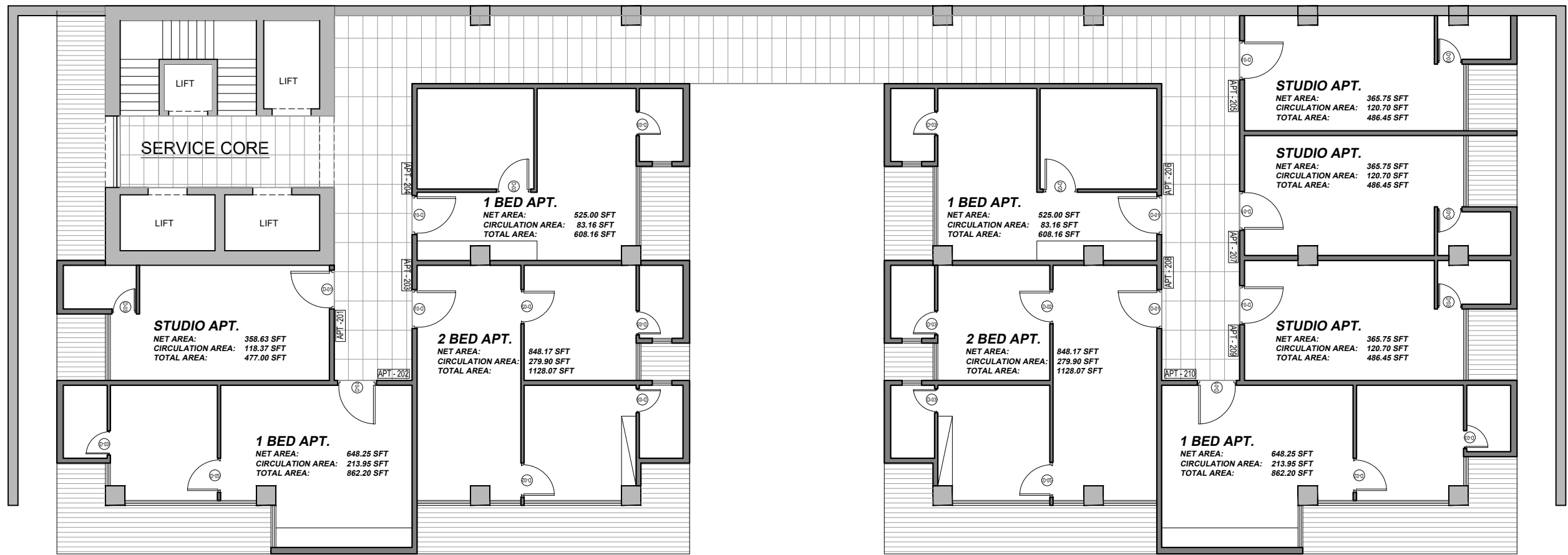
STAGE 01 2ND FLOOR AREA PLAN
